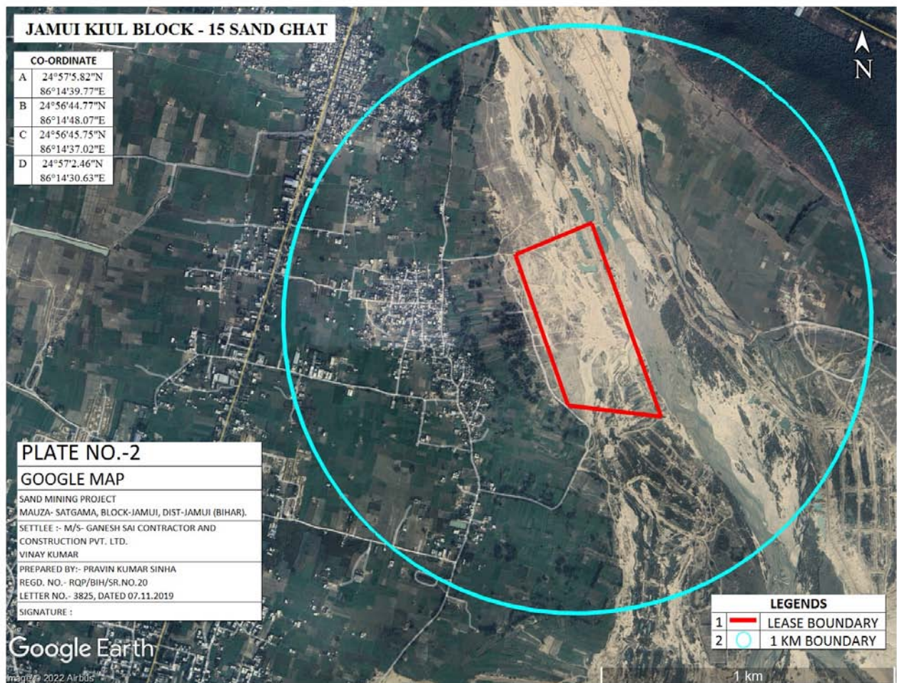
Figure 2.1:- Pillar Coordinate map of Jamui Kiul Block 15
